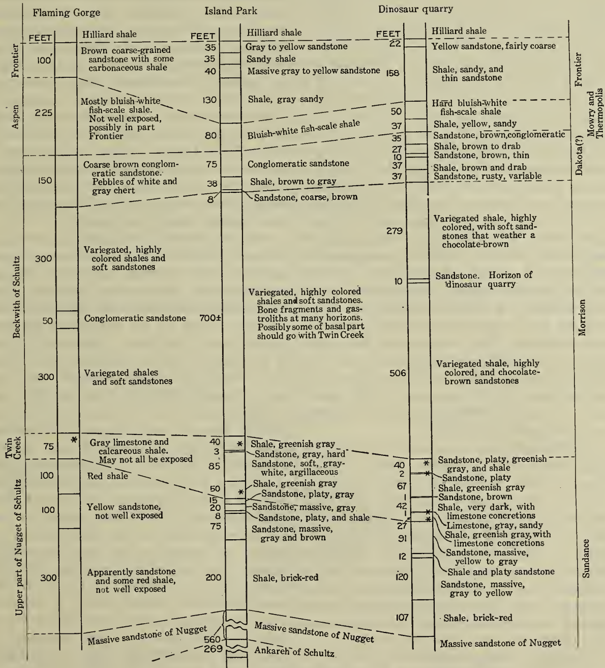
FIGURE 7.—Diagram showing correlation of sections near Flaming Gorge, Dagget County, and in Island Park and near the Carnegie Museum dinosaur quarry, Uinta County, Utah.
